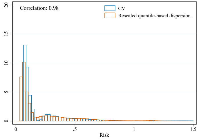
Figure G16: Comparing CV and quantile-based dispersion
