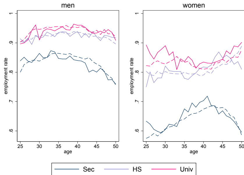
Figure 5: BHPS data and model predictions: employment of men and women over the lifecycle
