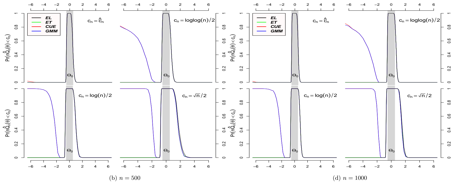
Figure 2: Coverage Probabilities for \{n\hat{Q}_n^j(\theta) \leq c_n^j\} Design 2.
